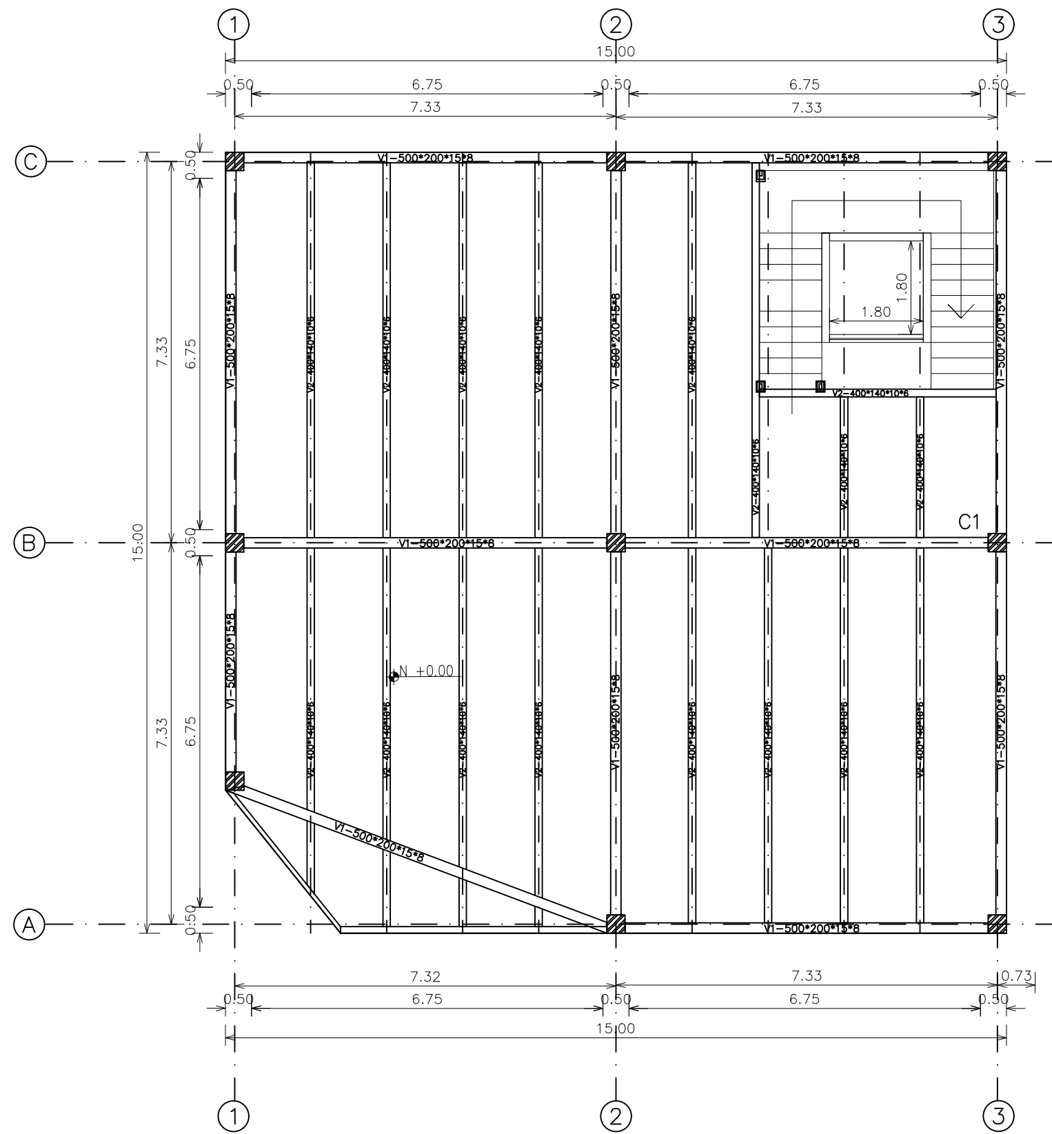
LOSA Nv.+3.53 Nv.+6.93 Nv.+10.33 Escala 1:100
